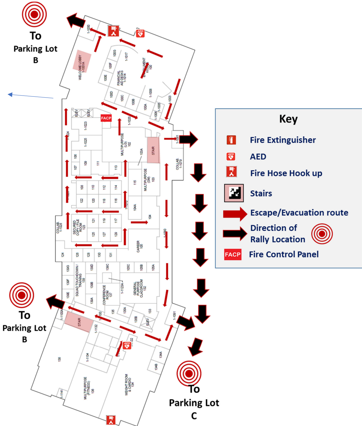
Figure 17. Wylie Campus, Campus Commons (Building B), Floor 1 Evacuation Map
