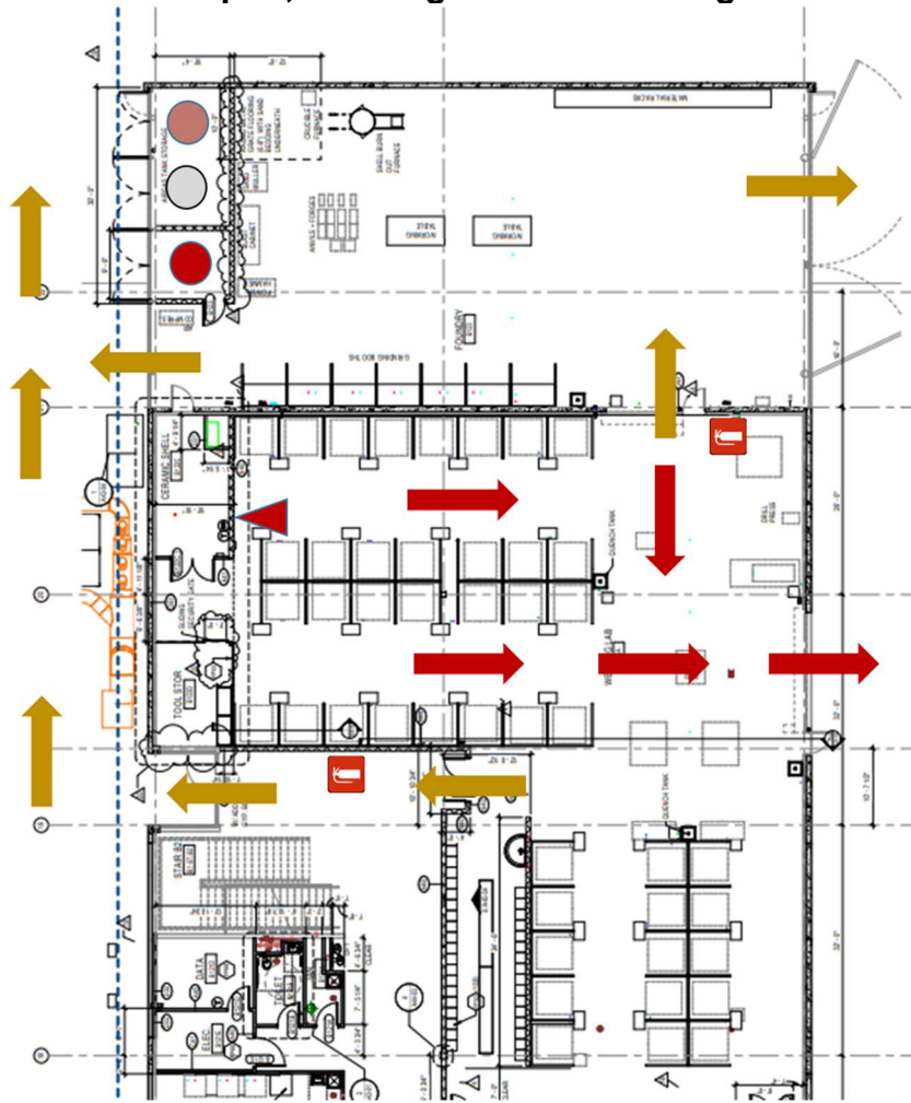
Figure 10. Technical Campus, Welding and Bulk Storage Area
