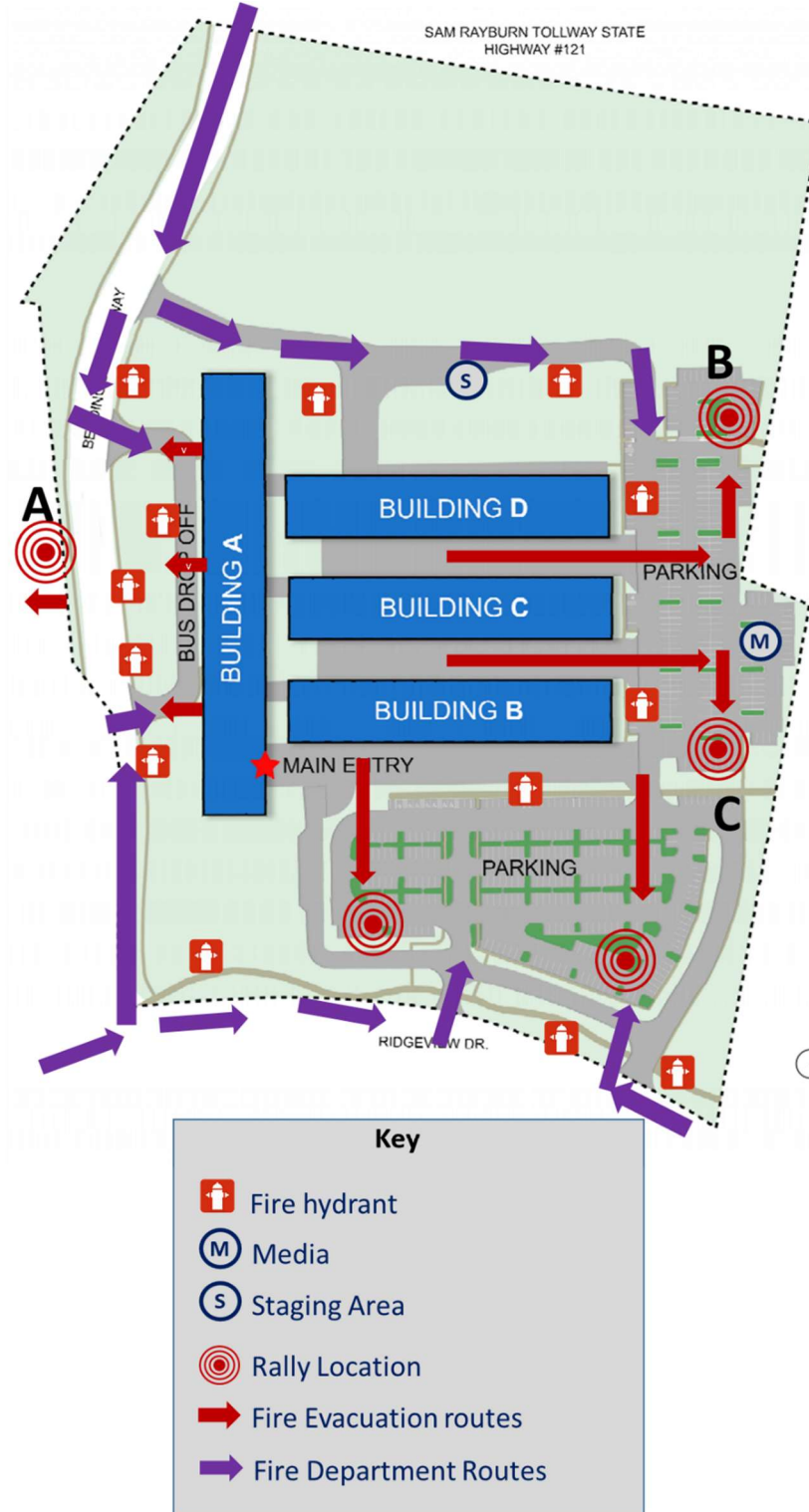
Figure 8. Technical Campus, Exterior Fire Assets
